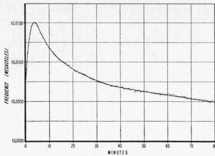
Figure 7. Warm-up stability curve of -hp- Model 608A 10-500 mc signal generator with frequency dial set for 10-megacycle output. Measurements made with -hp- Model 524A at 20-second intervals.
