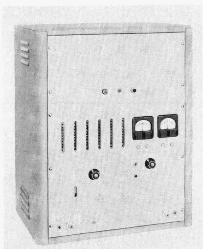
Figure 2. New -hp- Model 524A Frequency Counter.
