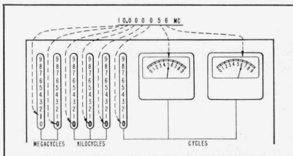
Figure 1. Display arrangement of new -hp- Model 524A Frequency Counter. Columns of neon tubes behind panel slots illuminate the proper numerals which are reverse-printed on transparent plastic. Example shown represents a frequency of 10,000,056 cps counted for period of one second. Maximum rate for instrument is 10 mc; maximum counting period is 10 seconds.
